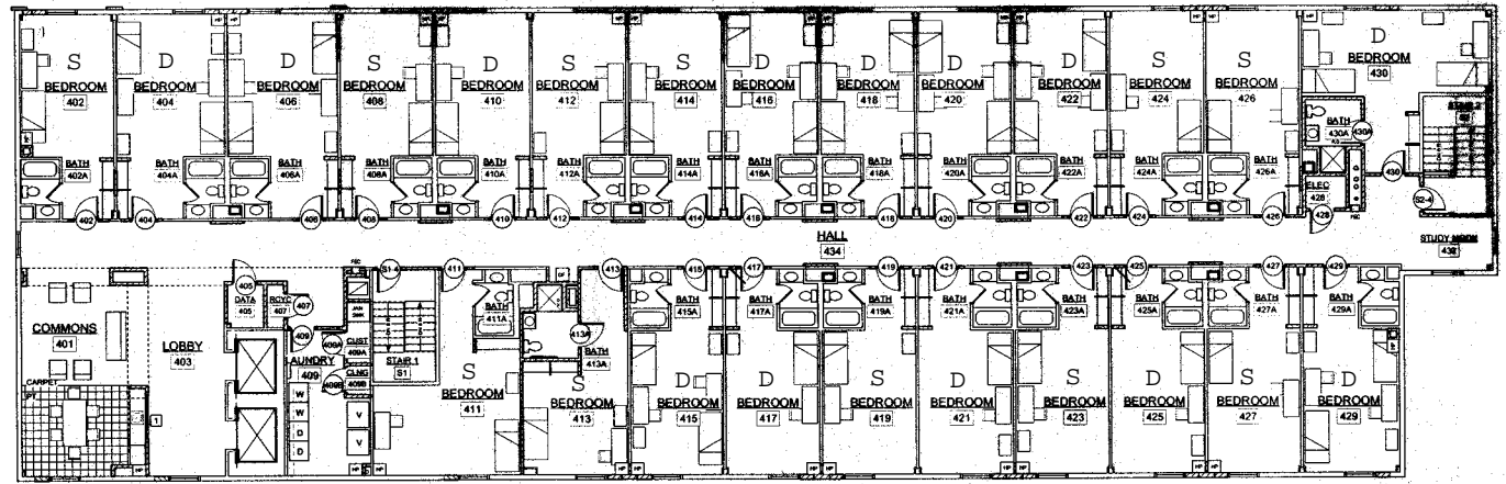
1 FOURTH FLOOR TOWER PLAN Scale: 1/8" = 1'-0"
