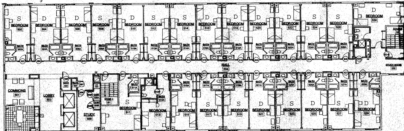
2 FIFTH FLOOR TOWER PLAN Scale: 1/8" = 1'-0"
