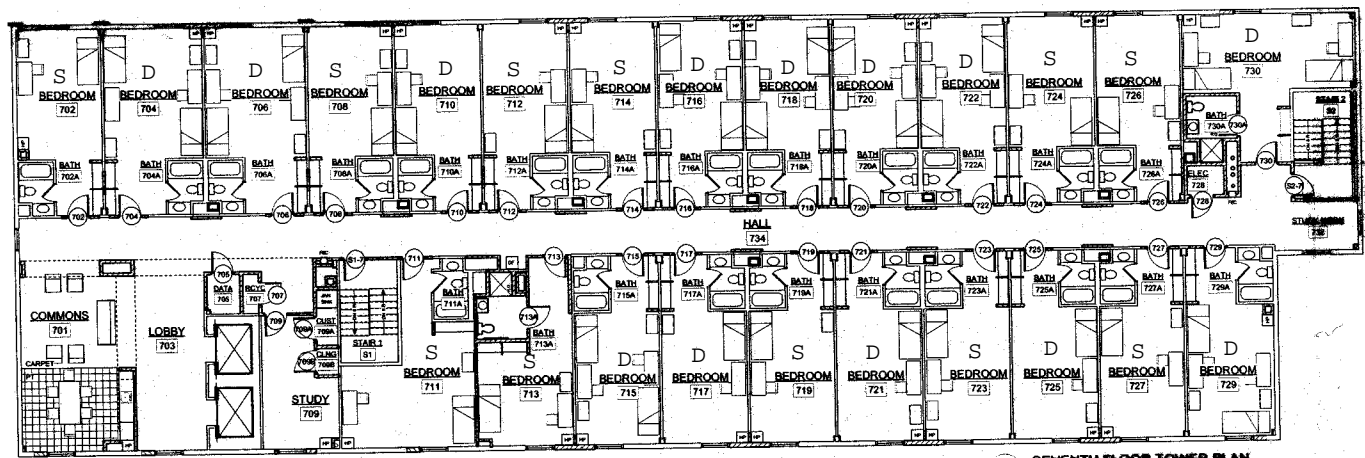
2 SEVENTH FLOOR TOWER PLAN Scale: 1/8" = 1'-0"
