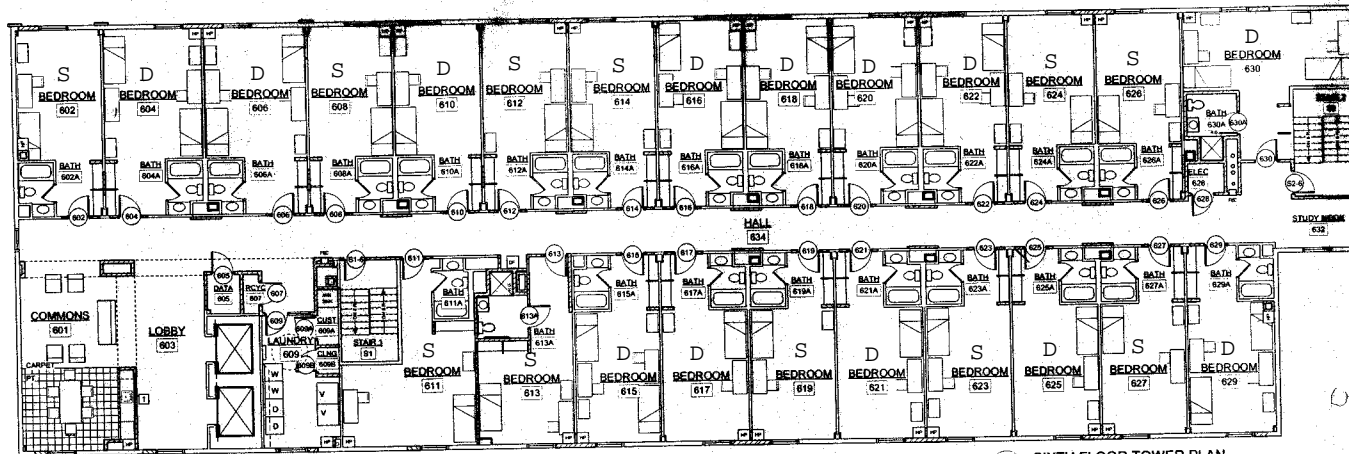
1 SIXTH FLOOR TOWER PLAN Scale: 1/8" = 1'-0"
